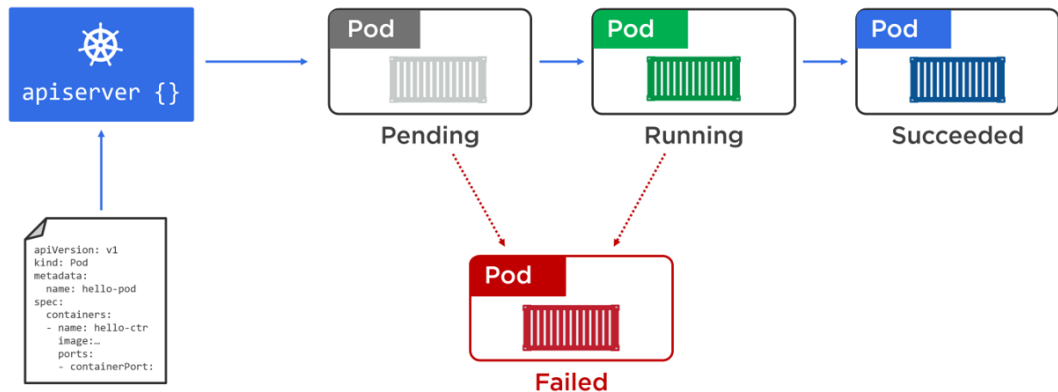
Figure 4.7 Pod lifecycle
