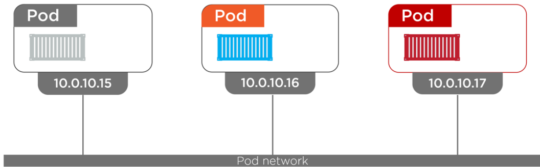
Figure 4.5 Inter-pod communication
