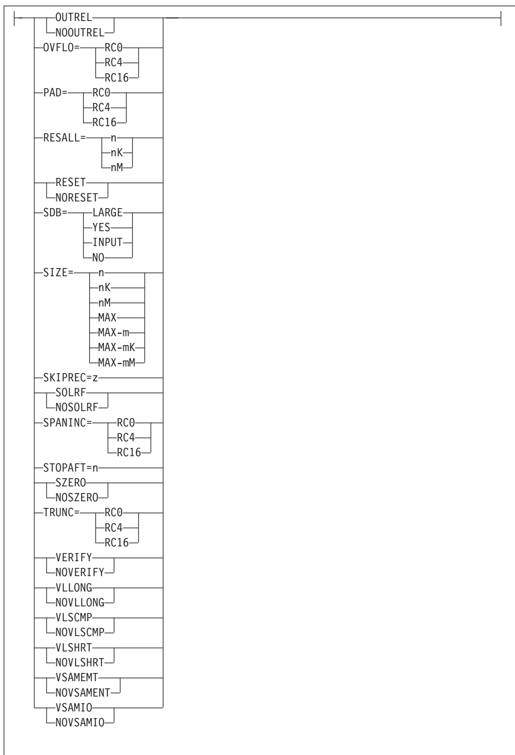
Figure 4. Syntax Diagram for EXEC PARM (Part 2 of 3)
