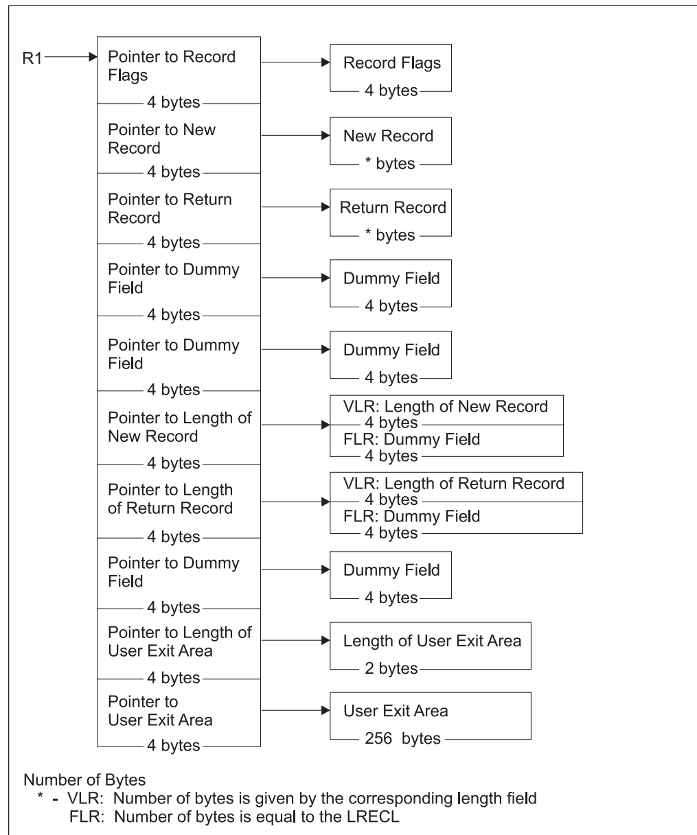
Figure 24. E15 DFSORT Interface with COBOL
