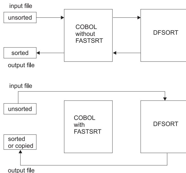
Figure 53. Faster Sorting with COBOL
