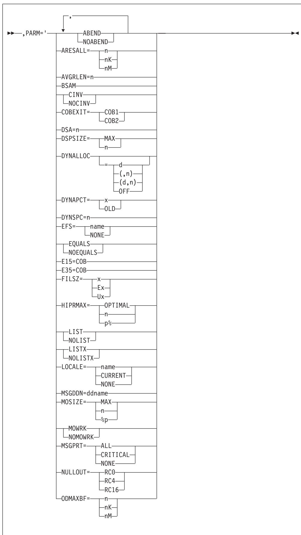
Figure 4. Syntax Diagram for EXEC PARM (Part 1 of 3)
