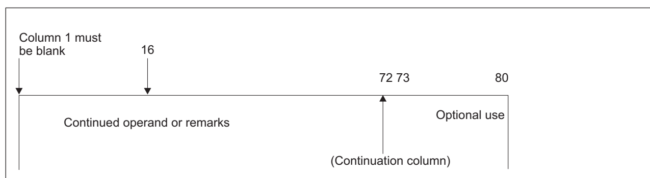
Figure 7. Continuation Line Format
