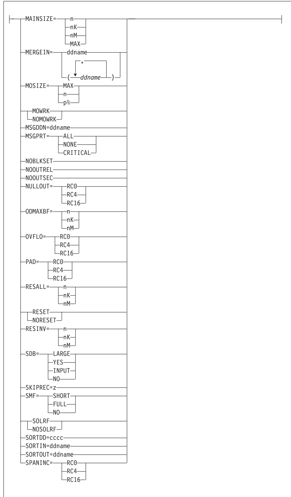
Figure 12. Syntax Diagram for the Option Control Statement (Part 2 of 3)
