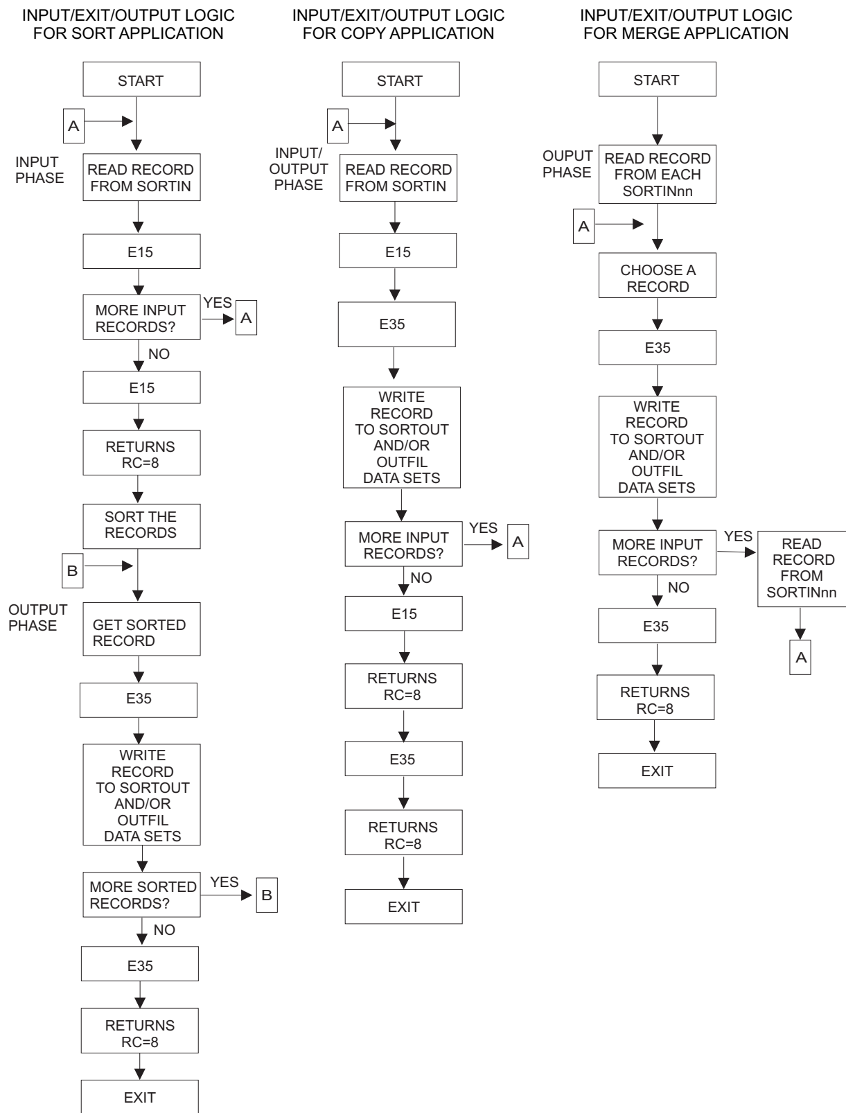
Figure 16. Examples of DFSORT Input/User Exit/Output Logic
