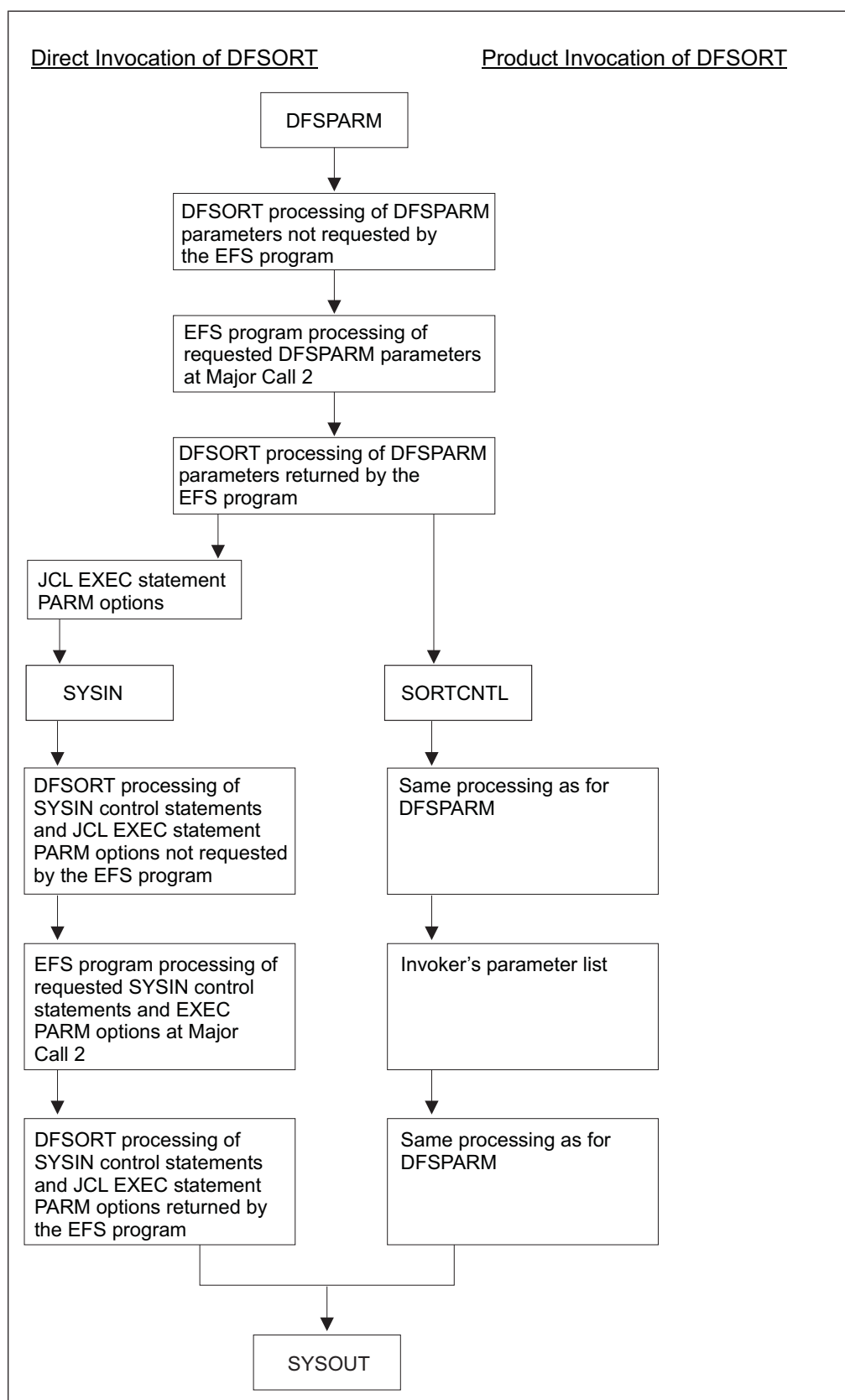
Figure 46. Control Statement Processing Sequence
