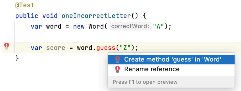
Figure 5.5 – Creating the Word class
