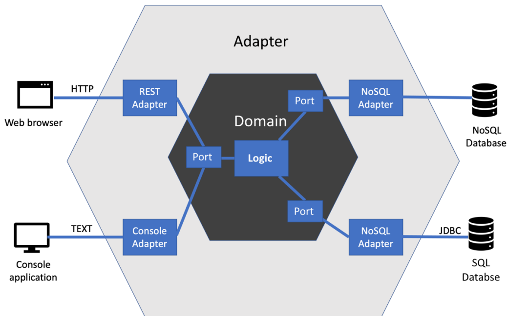
Figure 9.3 – Hexagonal architecture
