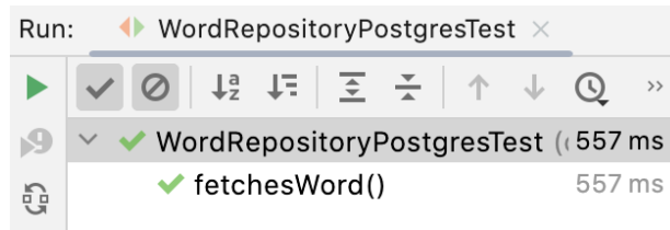
Figure 14.6 – Test passes
