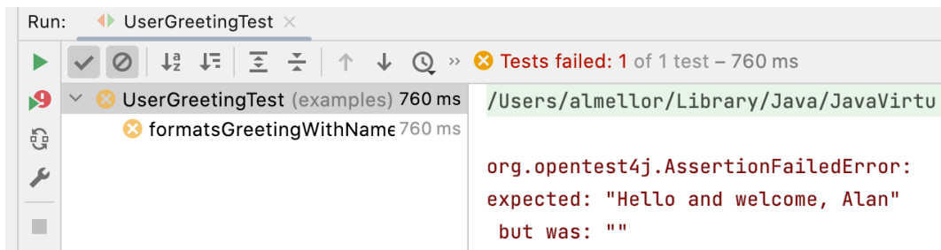
Figure 8.3 – Test failure
