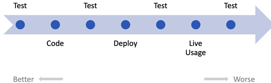
Figure 12.5 – Testing timeline
