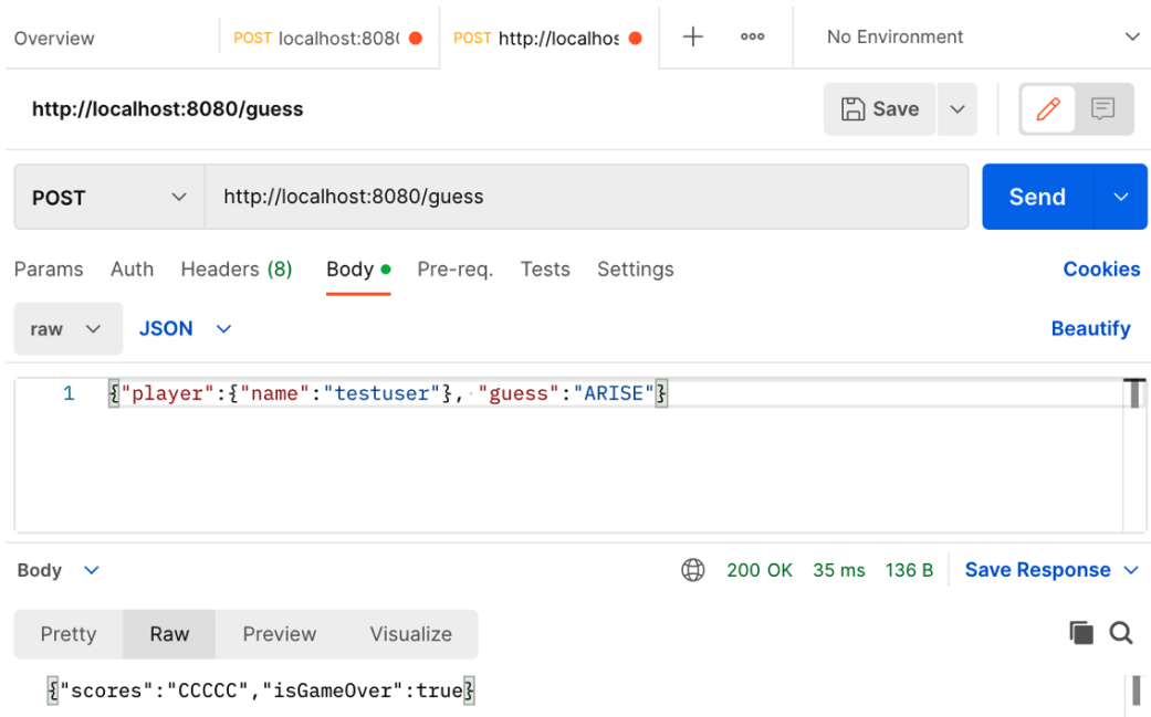
Figure 15.13 – A successful guess
