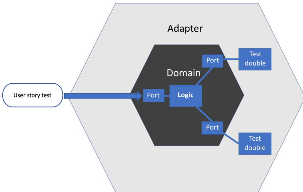
Figure 12.10 – Testing user stories
