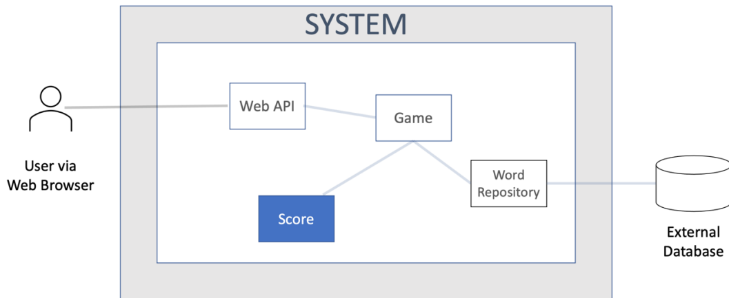
Figure 12.6 – Inside-out development
