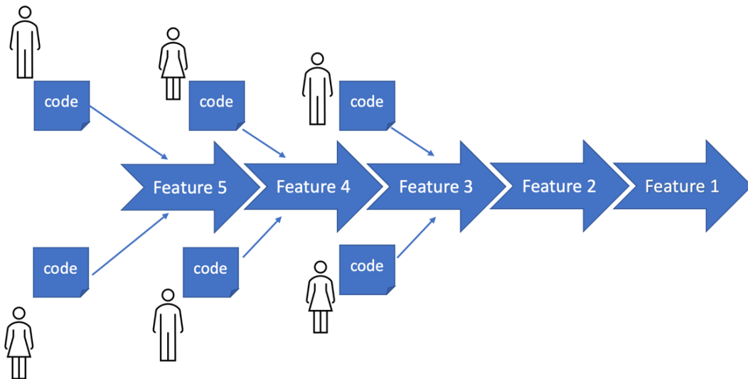
Figure 10.7 – Continuous integration
