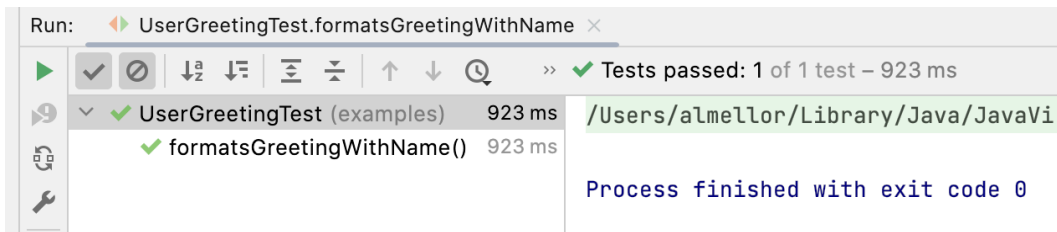
Figure 8.7 – Test pass
