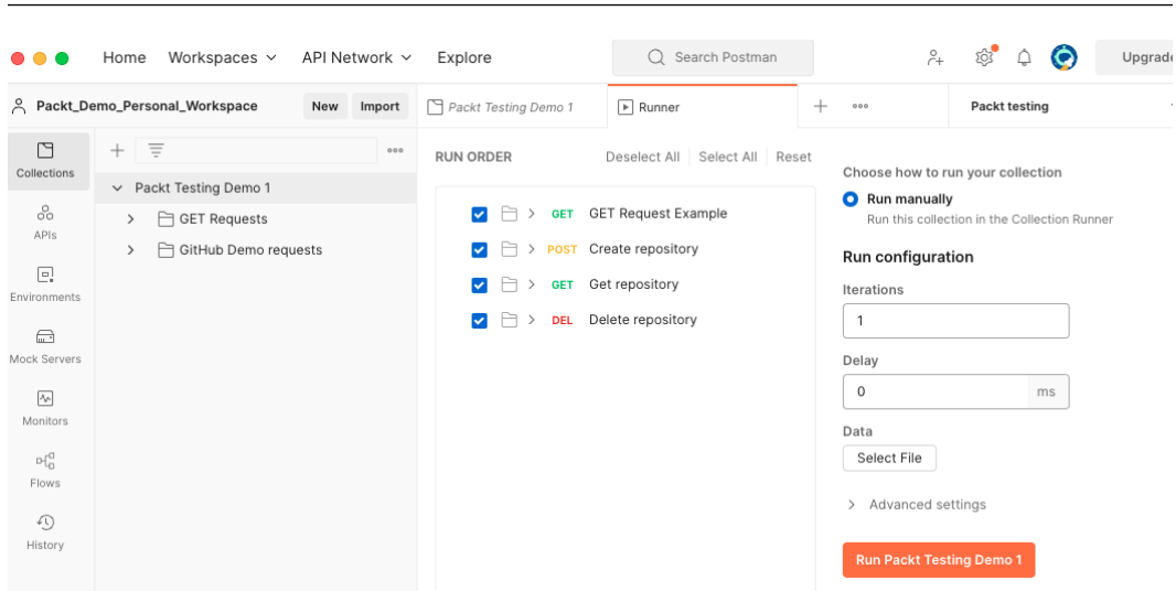
Figure 7.18 – Collection runner window
