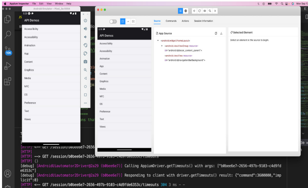
Figure 6.13 – Test application loaded in Appium Inspector and the emulator
