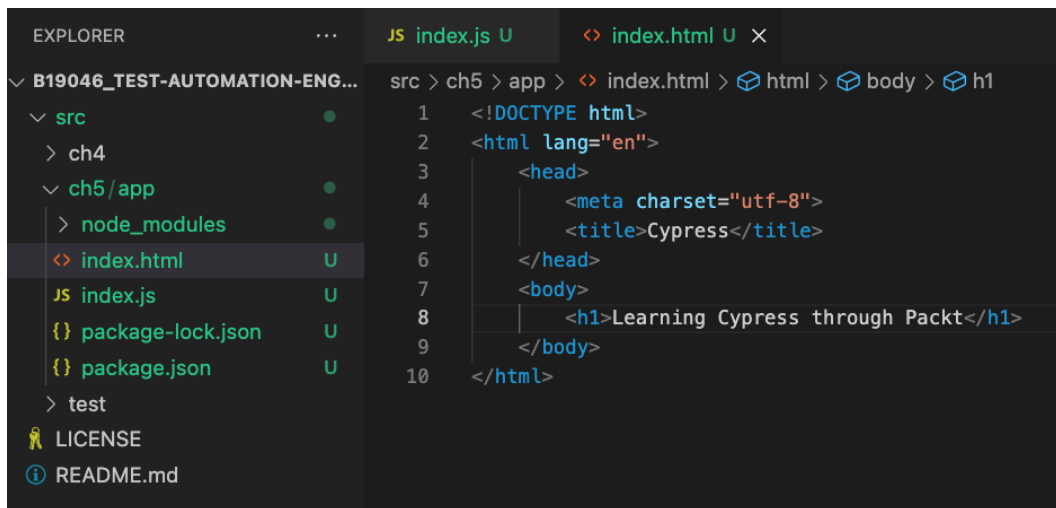
Figure 5.4 – Creating an index.html file
