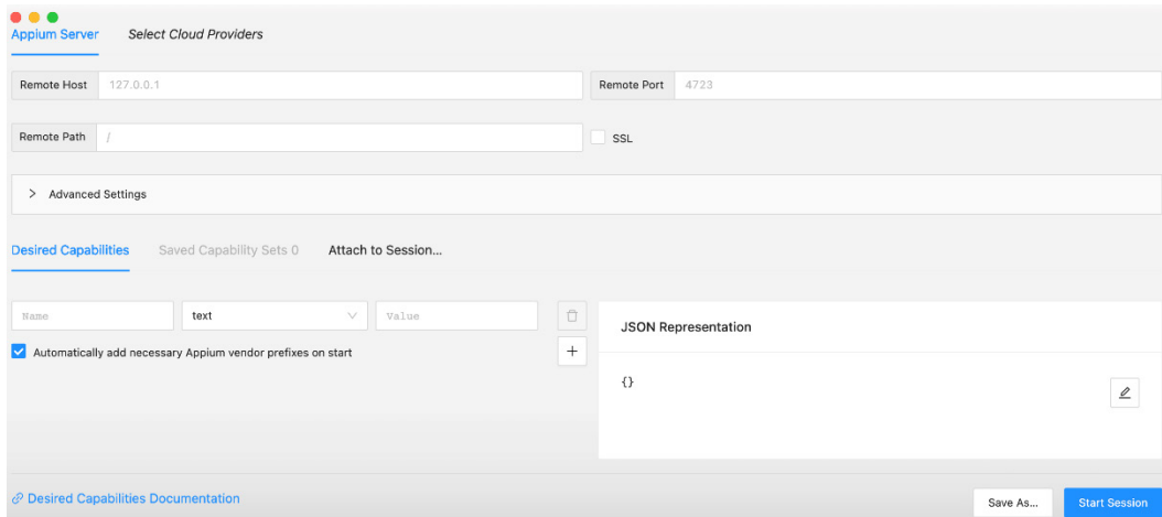
Figure 6.11 – Appium Inspector tool
