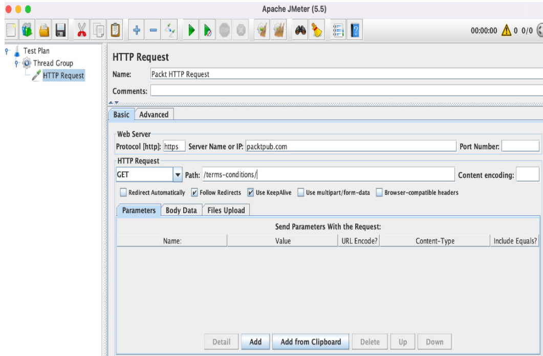
Figure 8.7 – Configuring an HTTP sampler
