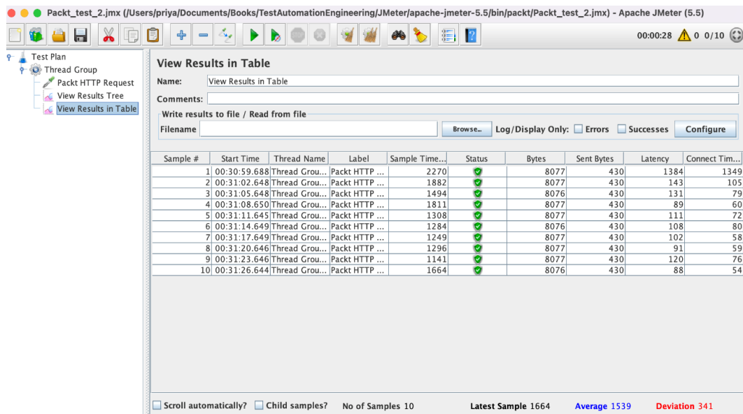
Figure 8.9 – Test run results
