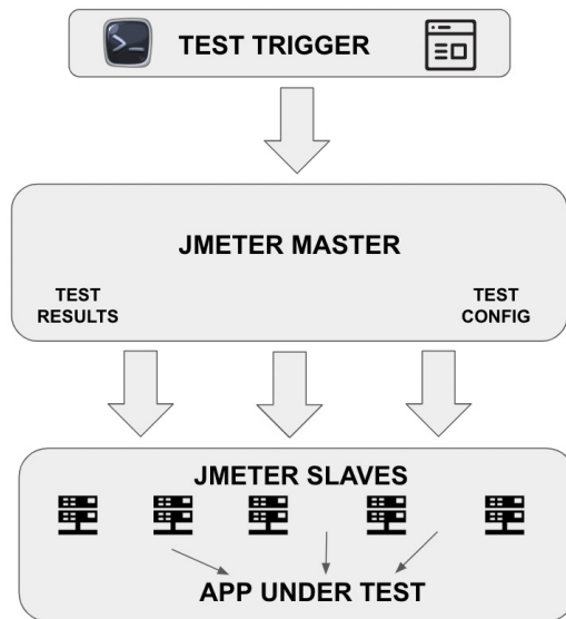
Figure 3.22 – JMeter architecture/components
