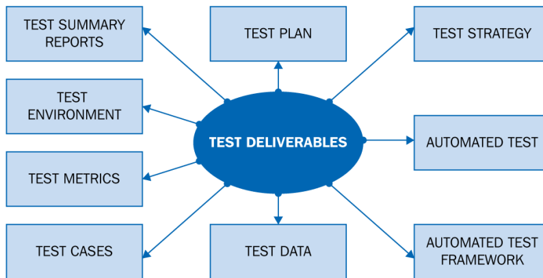
Figure 1.1 – Testing deliverables
