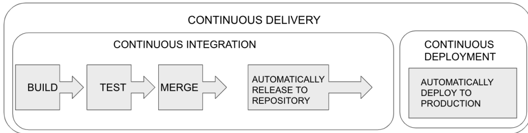
Figure 9.1 – CI/CD
