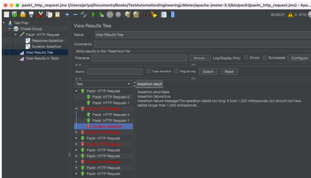
Figure 8.11 – Assertion results
