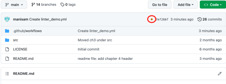
Figure 9.6 – Workflow status
