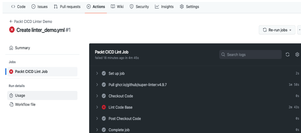
Figure 9.7 – Workflow results
