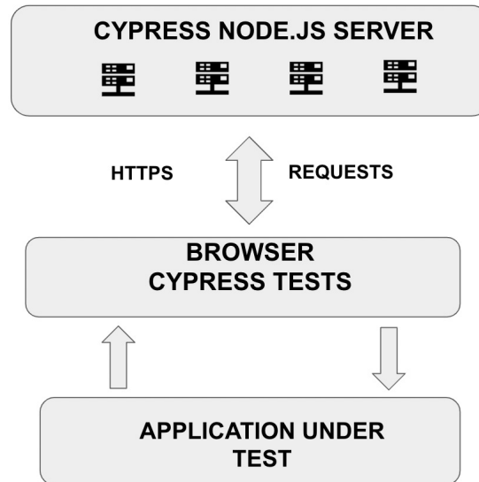
Figure 3.21 – Cypress architecture/components
