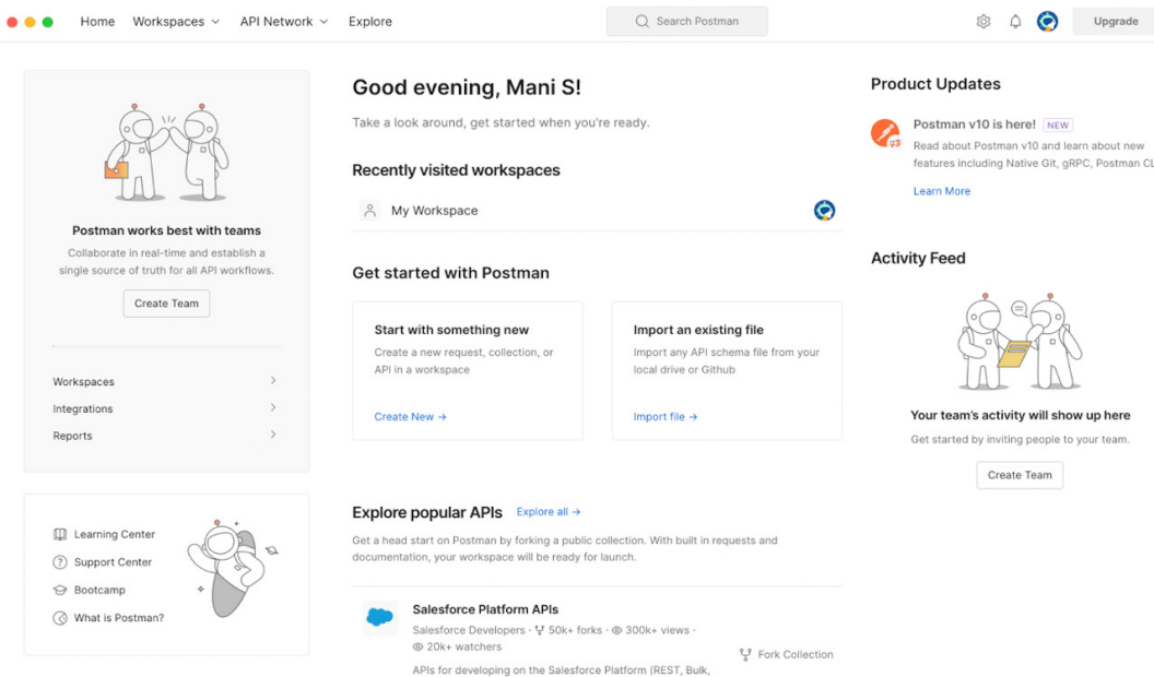
Figure 7.1 – Postman application
