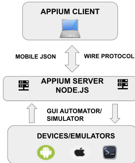
Figure 3.20 – Appium architecture/components
