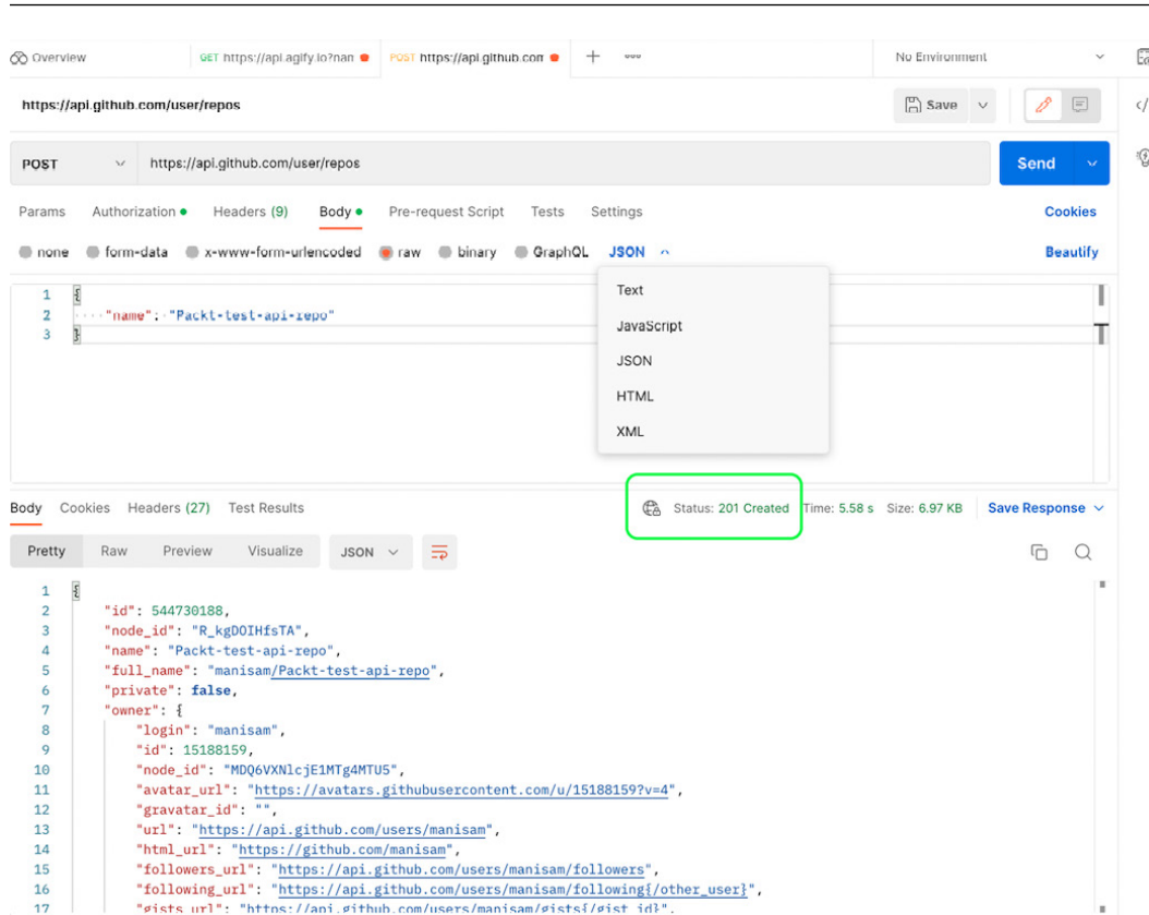
Figure 7.9 – POST API request body type
