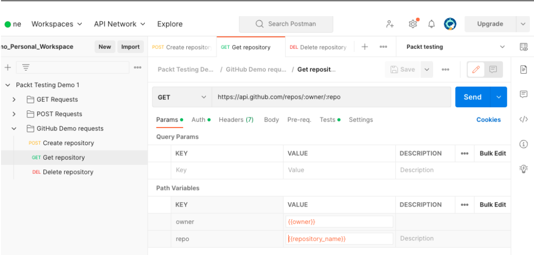
Figure 7.17 – Chaining API requests
