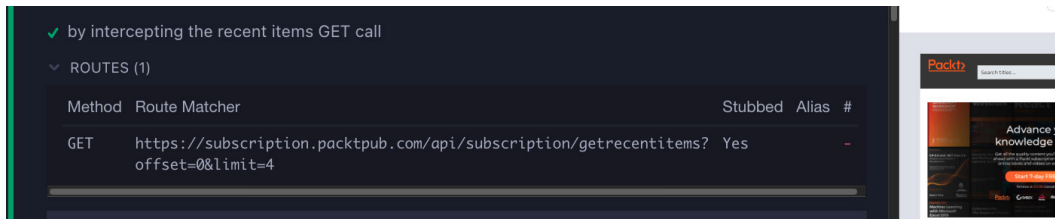
Figure 5.22 – Intercept results
