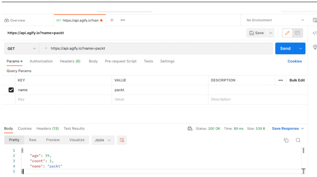
Figure 7.7 – API request with a query parameter
