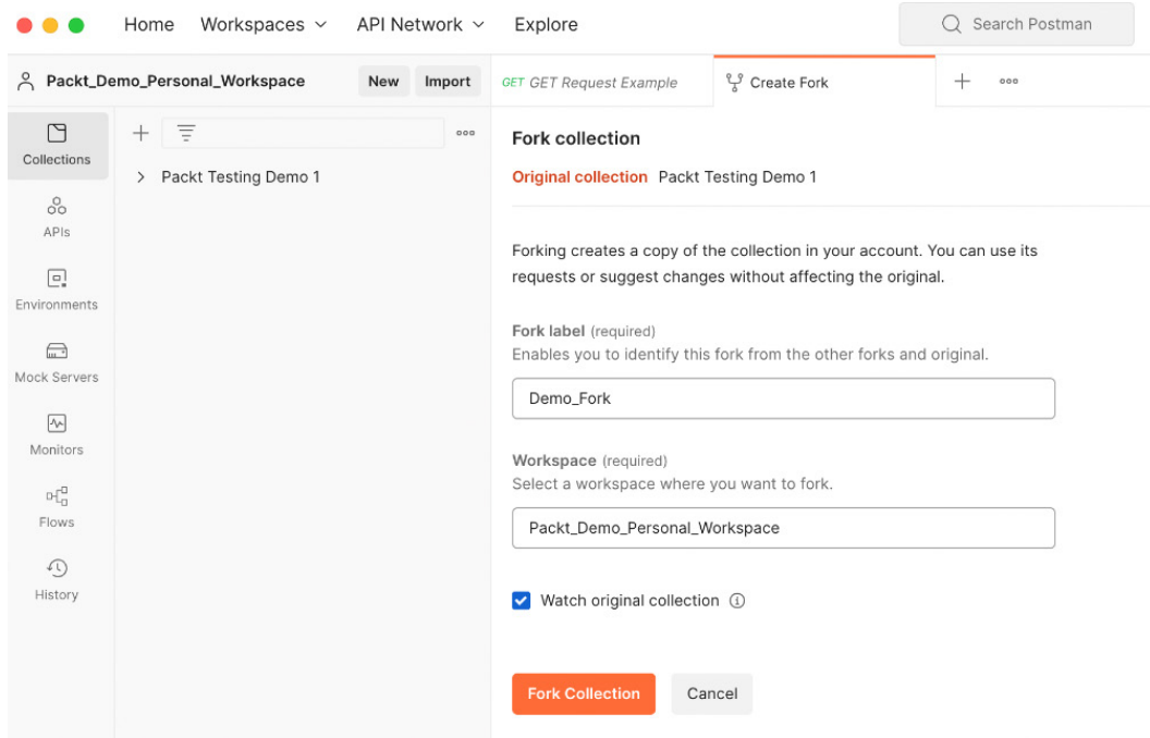
Figure 7.12 – Forking a collection
