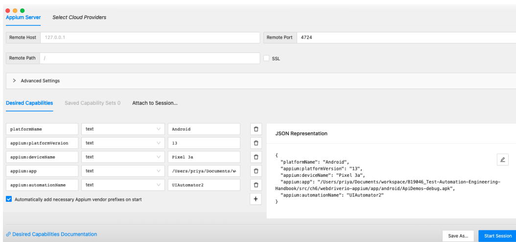
Figure 6.12 – Appium Inspector configuration
