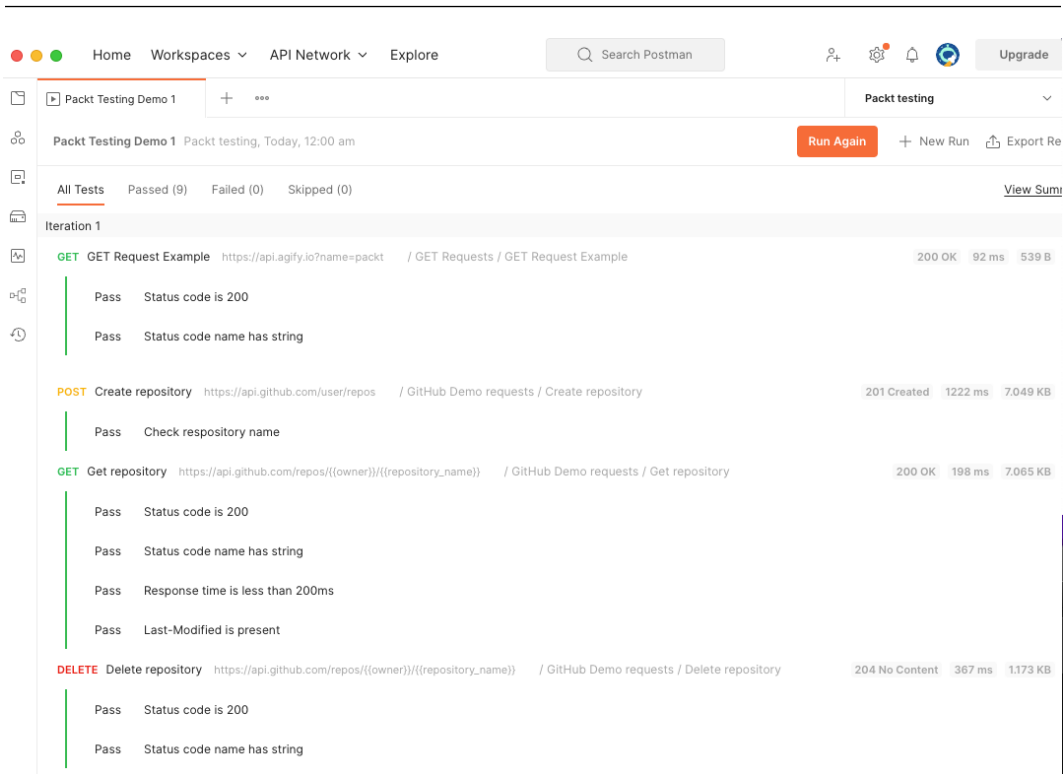
Figure 7.19 – Test results summary
