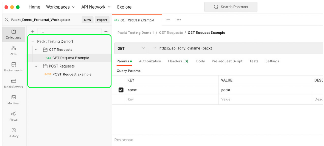
Figure 7.10 – Collections
