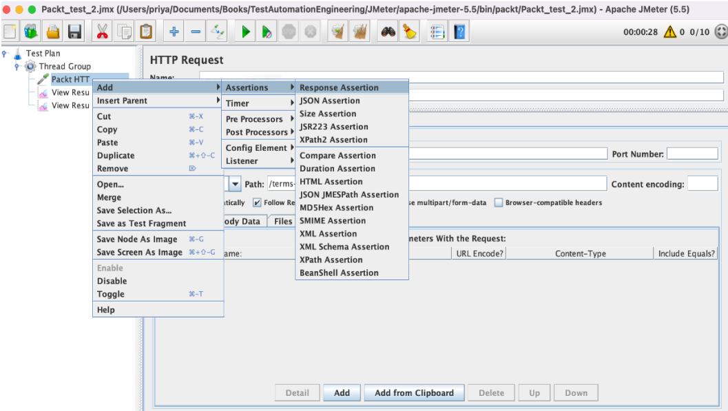
Figure 8.10 – Adding assertions
