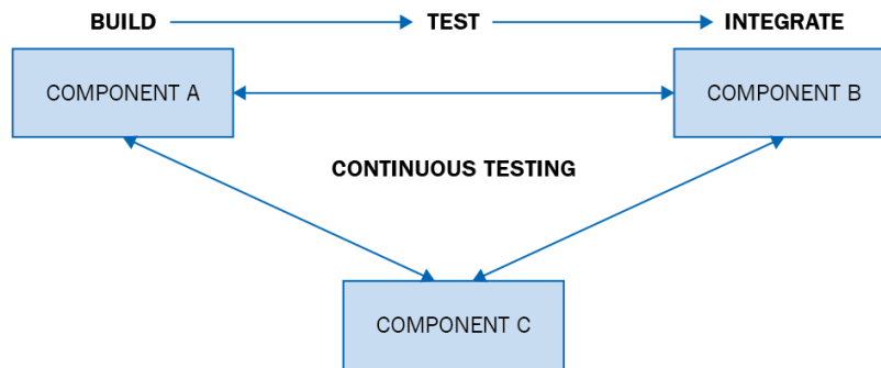
Figure 1.2 – Continuous testing
