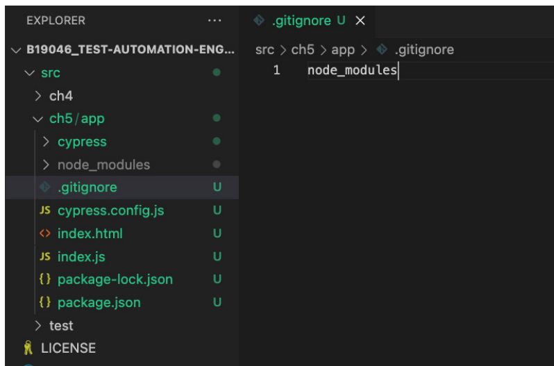
Figure 5.23 – .gitignore file
