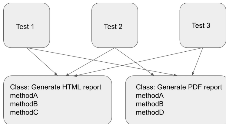
Figure 10.1 – Code duplication
