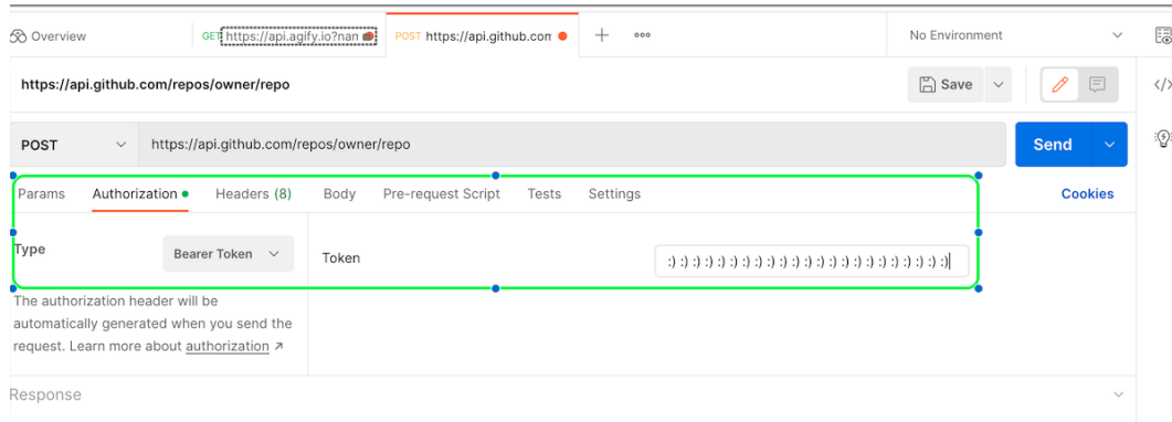
Figure 7.8 – POST API request authorization
