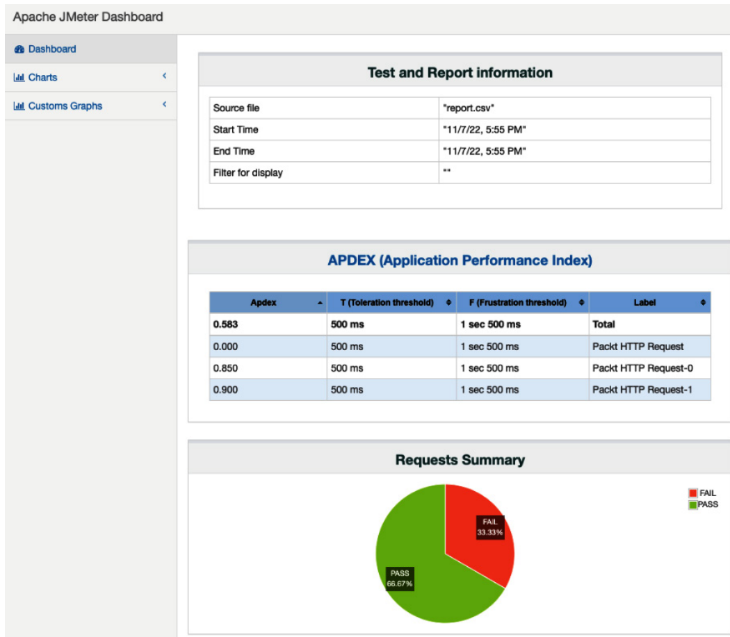
Figure 8.14 – JMeter Dashboard report
