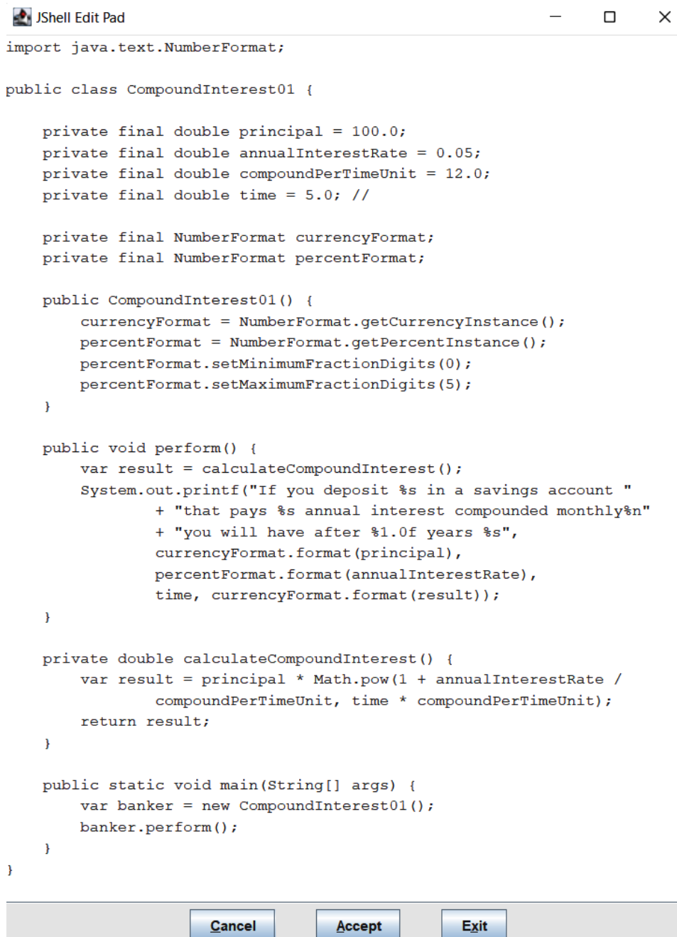
Figure 2.4 – The program after being pasted into the default JShell editor
