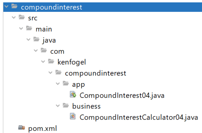
Figure 3.4 – Basic Maven file structure
