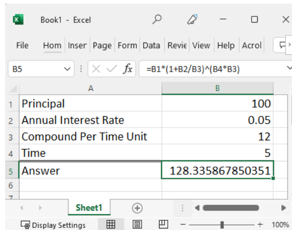
Figure 2.3 – The compound interest calculation in Excel
