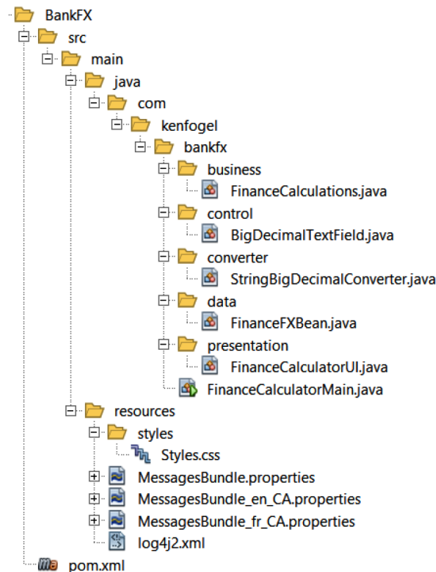
Figure 13.7 – The JavaFX program layout
