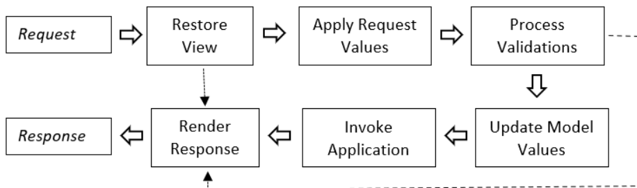
Figure 15.4 – The Faces life cycle
