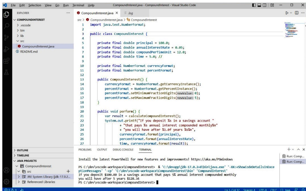
Figure 2.15 – The compound interest program in VS Code
