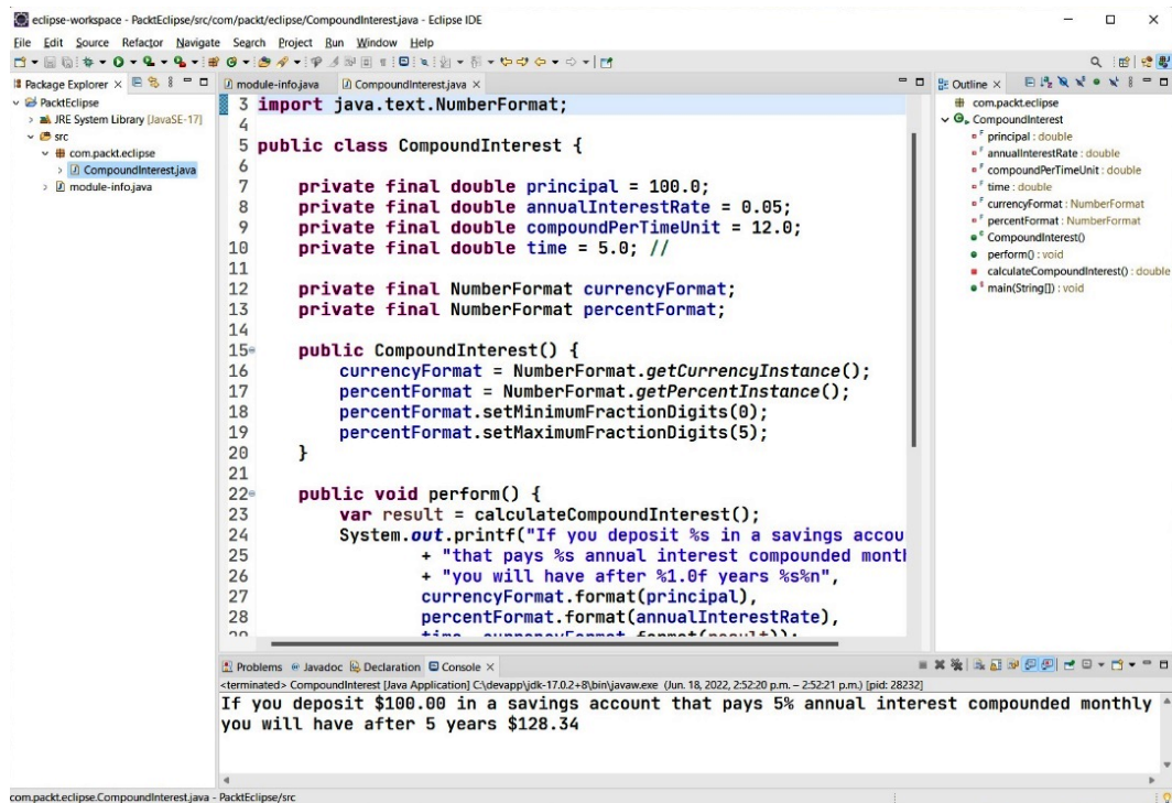
Figure 2.13 – The compound interest program in Eclipse
