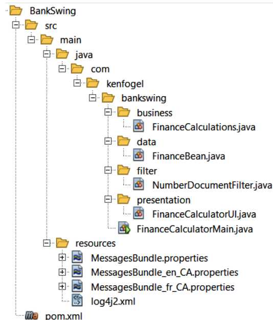
Figure 13.5 – The Swing project layout
