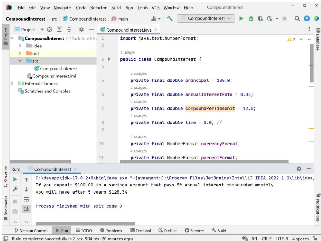
Figure 2.16 – The compound interest program in IntelliJ IDEA
