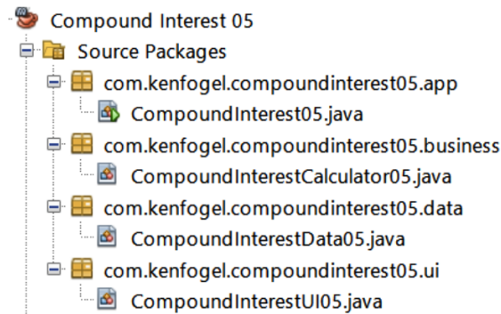
Figure 10.1 – Class organization for the separation of concerns principle
