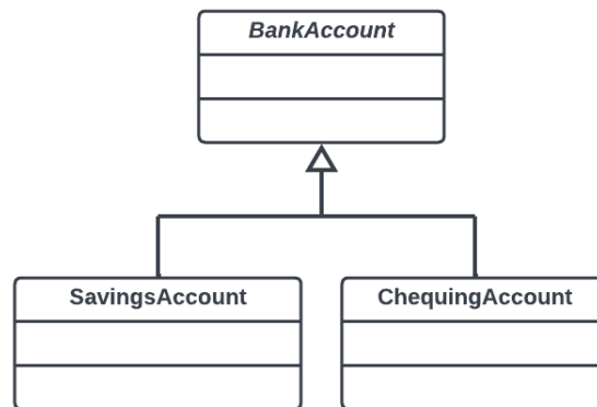
Figure 6.1 – The BankAccount inheritance hierarchy
