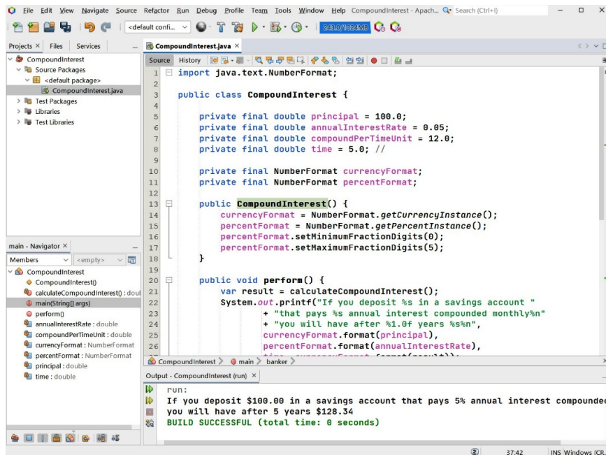
Figure 2.14 – The compound interest program in NetBeans
