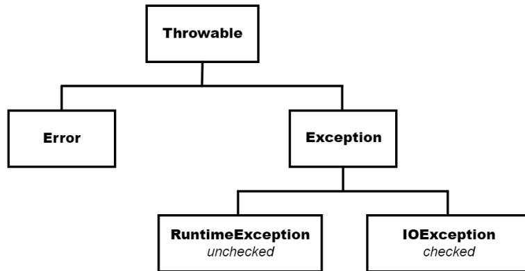
Figure 7.1 – The exception hierarchy
