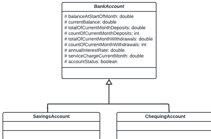
Figure 6.2 – The BankAccount class fields
