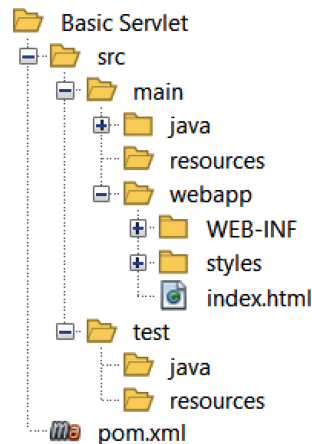
Figure 14.3 – The required folders for a Jakarta EE app being built with Maven
