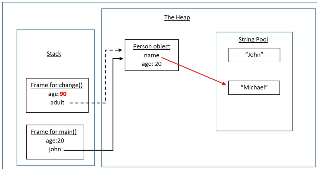
Figure 2.8 – The stack and heap as the change() method is exiting
