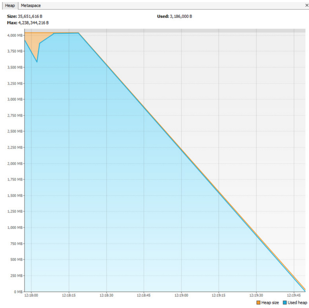
Figure 7.2 – Heap memory footprint
