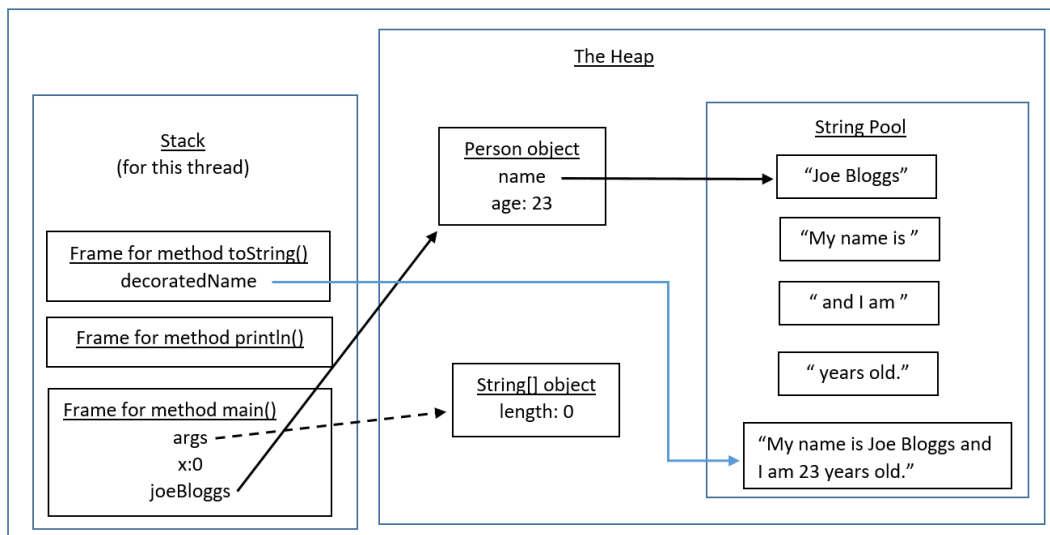
Figure 2.4 – A stack and heap representation of the code in Figure 2.3
