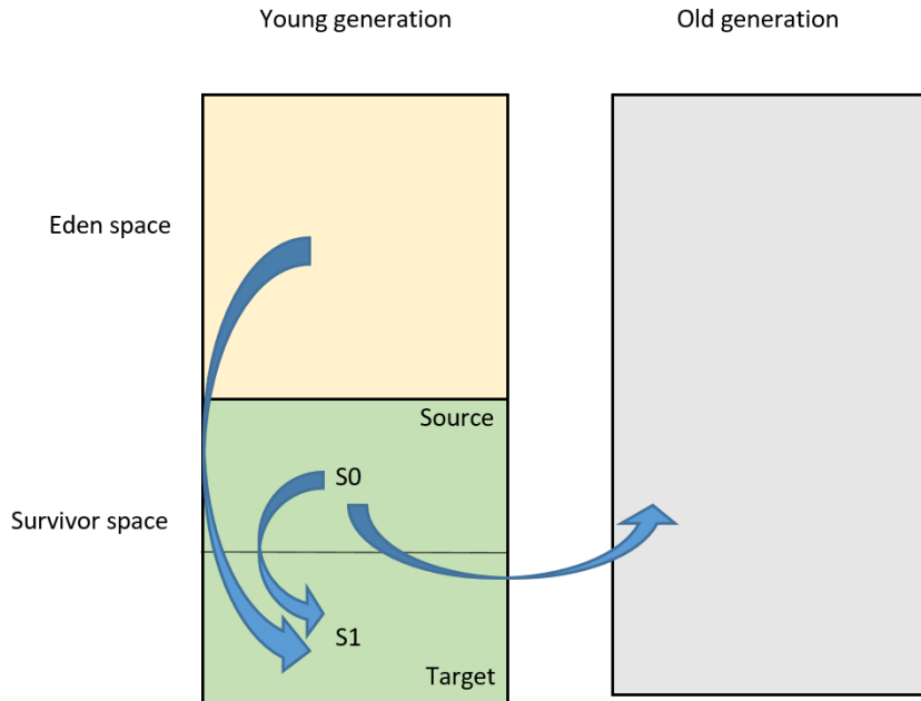
Figure 3.4 – Minor garbage collection with S1 as the target space
