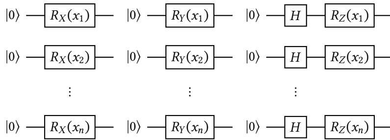
Figure 9.6: Angle encoding for an input (x_1, \dots, x_n) using different rotation gates
