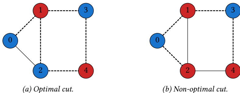
Figure 3.2: Two different cuts of the same graph
