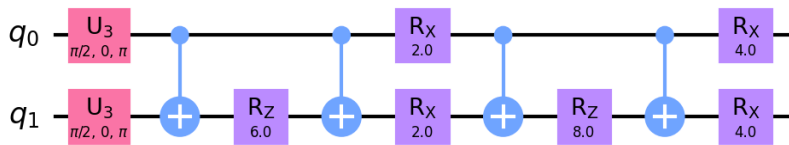
Figure 5.6: QAOA circuit for H_1 = Z_0Z_1 with p = 2
