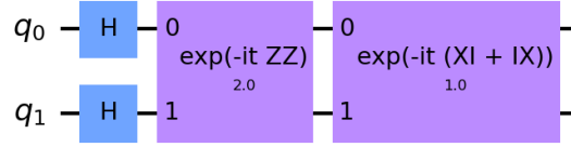
Figure 5.4: QAOA circuit for H_1 = Z_0Z_1
