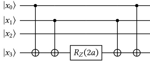
Figure 5.3: Implementation of e^{-iaZ_0Z_1Z_3}
