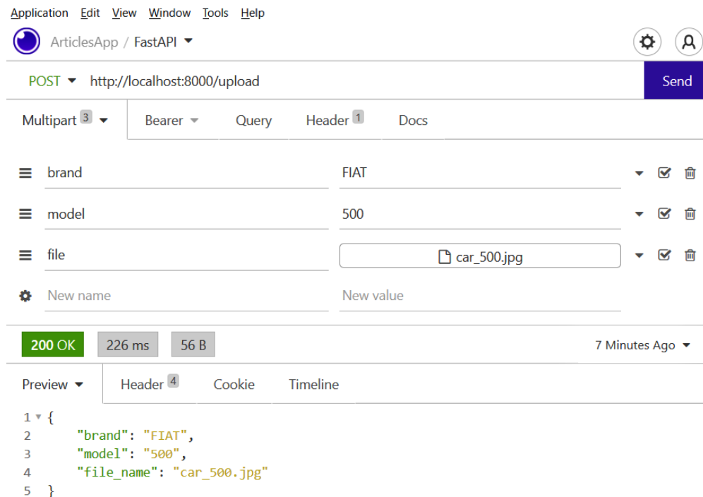
Figure 3.3 – Testing file uploads and form fields with the Insomnia REST client
