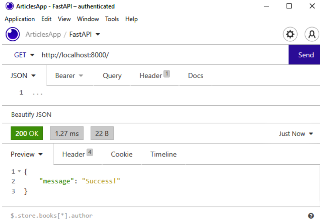
Figure 3.1 – Testing the root endpoint with Insomnia
