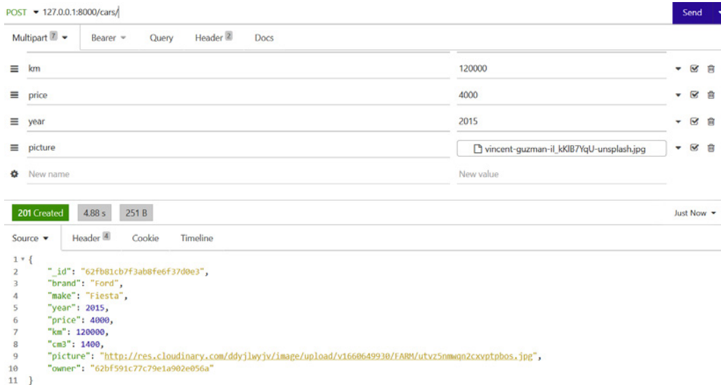
Figure 8.3 – Insomnia REST client performing a POST request
