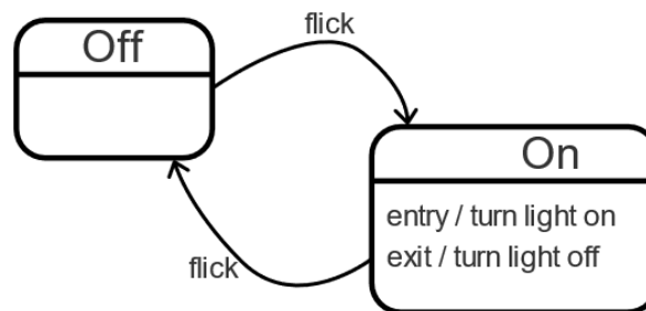
Figure 7.1 – Simple statechart drawing of a light switch
