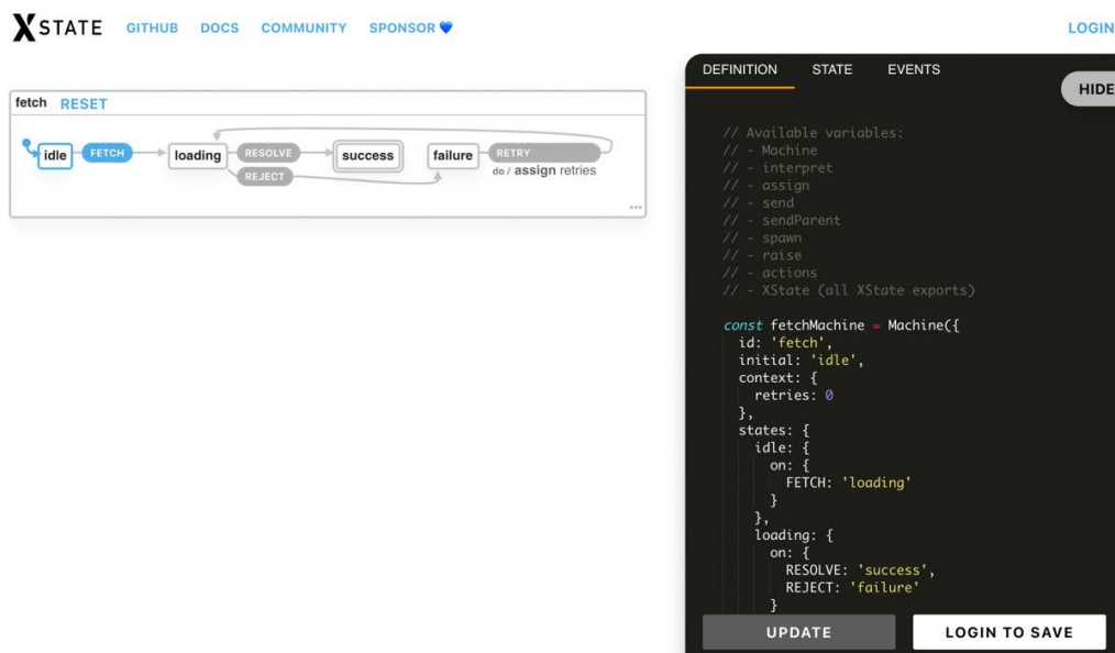
Figure 7.3 – Screenshot of the XState visualizer
