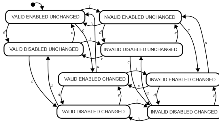
Figure 7.2 – Complex state chart
