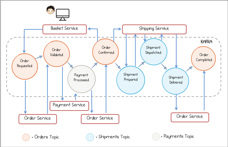
Figure 11-3. Here each circle represents an event; the color of the circle designates the topic it is in; a workflow evolves from Order Requested through to Order Completed; on the way, four services perform different state transitions in topics they are “single writer” to; the overall workflow spans them all
