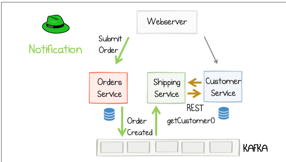
Figure 5-4. An event-driven version of the system described in Figure 5-3; in this configuration the events are used only as a means of notification: the orders service notifies the shipping service via Kafka
