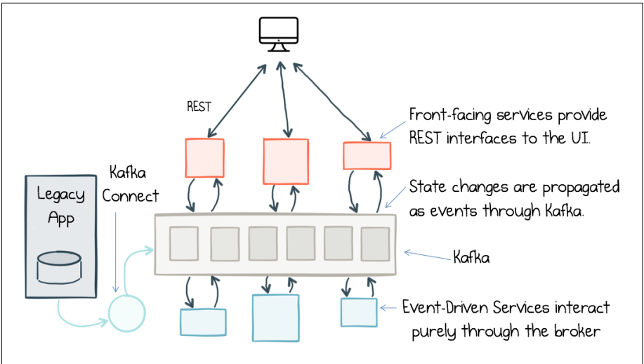
Figure 5-9. A very simple event-driven services example, data is imported from a legacy application via the Connect API; user-facing services provide REST APIs to the UI; state changes are journaled to Kafka as events. at the bottom, business processing is performed via Event Collaboration
