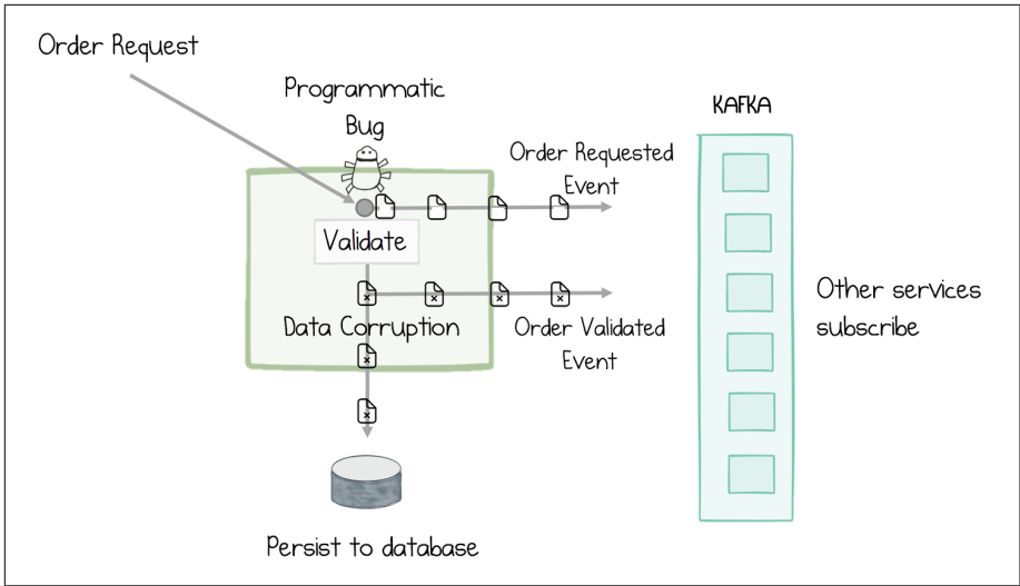
Figure 7-3. Adding Kafka and an Event Sourcing approach to the system described in Figure 7-2 ensures that the original events are preserved before the code, and bug, execute
