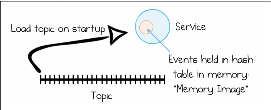
Figure 7-13. A MemoryImage is a simple “cache” of an entire topic loaded into a service so it can be referenced locally
