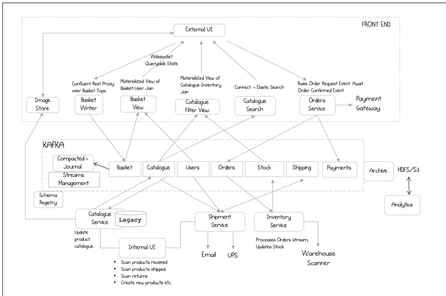
Figure 15-8. A more holistic streaming ecosystem
