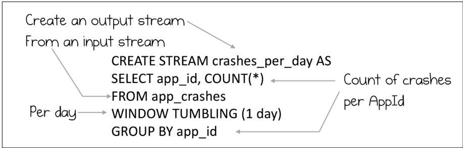
Figure 2-2. A simple KSQL query that evaluates crashes per day
